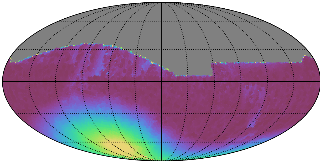
baseline_v2.1_10yrs All sky z band: Min moonDistance
