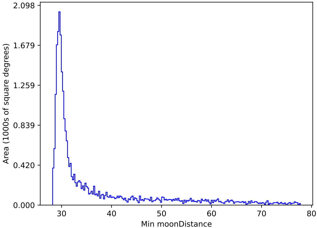
baseline_v2.1_10yrs All sky z band: Min moonDistance
