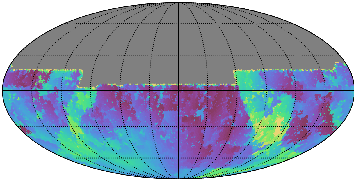
baseline_v2.1_10yrs All sky u band: Min moonDistance
