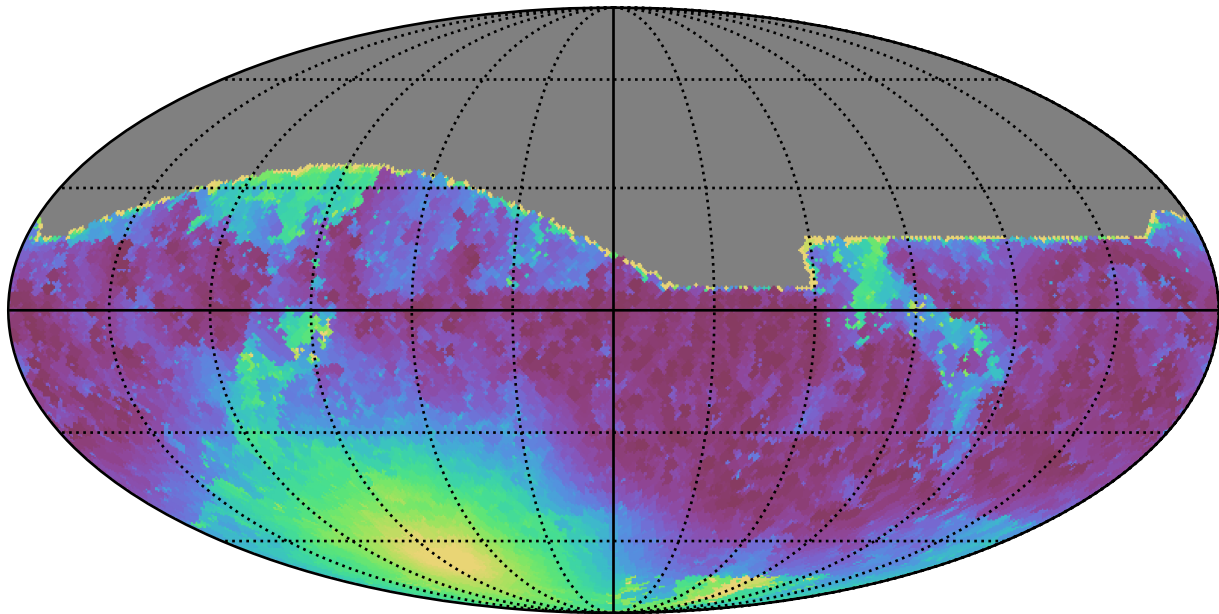
baseline_v2.1_10yrs All sky r band: Min moonDistance
