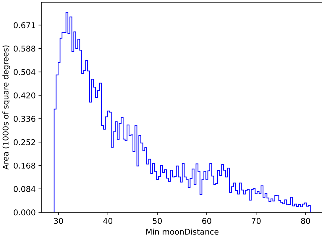
baseline_v2.1_10yrs All sky r band: Min moonDistance
