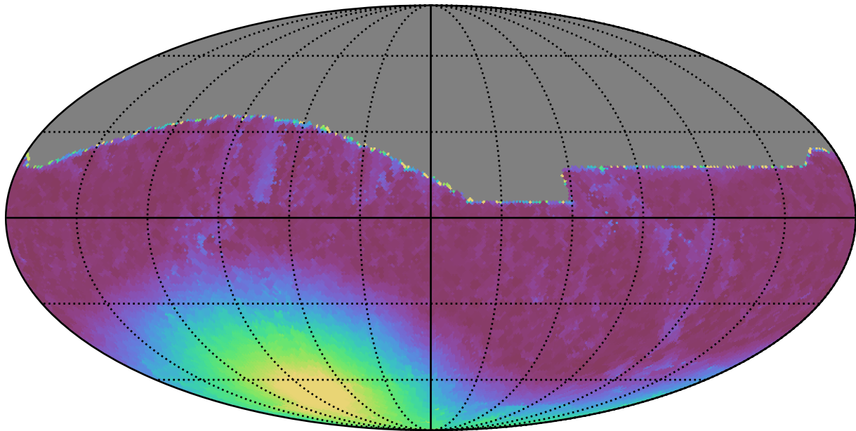
baseline_v2.1_10yrs All sky i band: Min moonDistance
