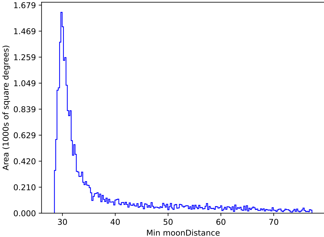
baseline_v2.1_10yrs All sky i band: Min moonDistance
