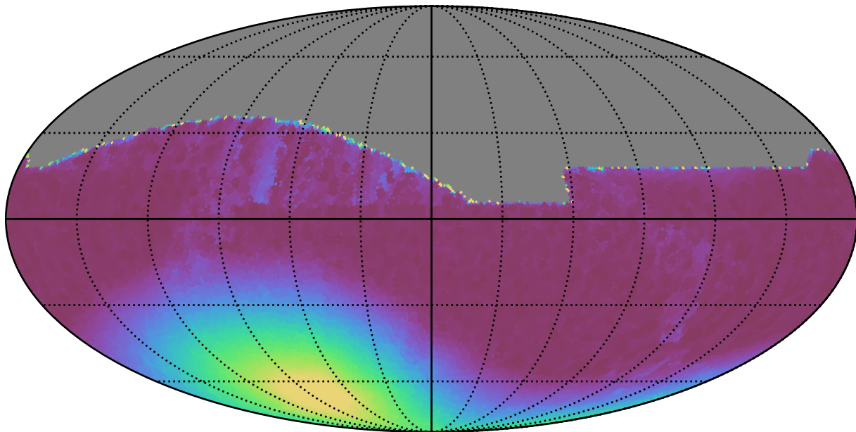
baseline_v2.1_10yrs All sky all bands: Min moonDistance
