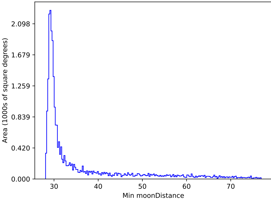
baseline_v2.1_10yrs All sky all bands: Min moonDistance
