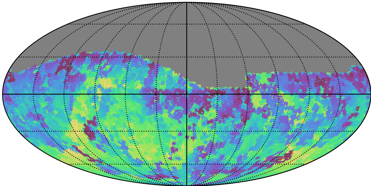
baseline_v2.1_10yrs Yr 1 z band: Min fiveSigmaDepth
