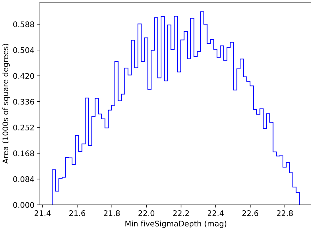
baseline_v2.1_10yrs Yr 1 z band: Min fiveSigmaDepth
