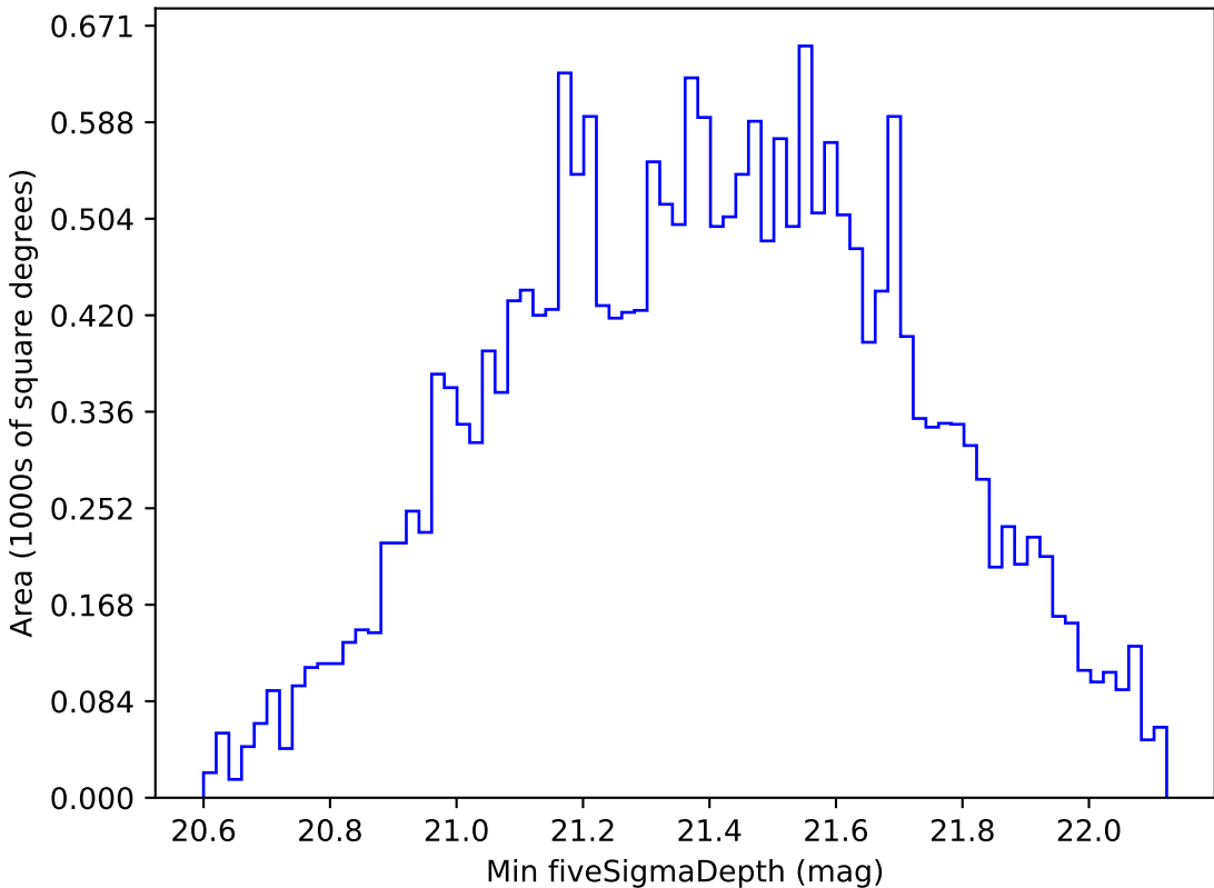
baseline_v2.1_10yrs Yr 1 y band: Min fiveSigmaDepth
