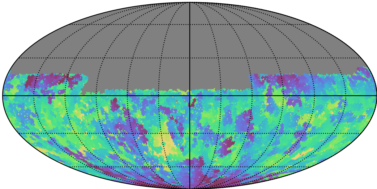
baseline_v2.1_10yrs Yr 1 u band: Min fiveSigmaDepth
