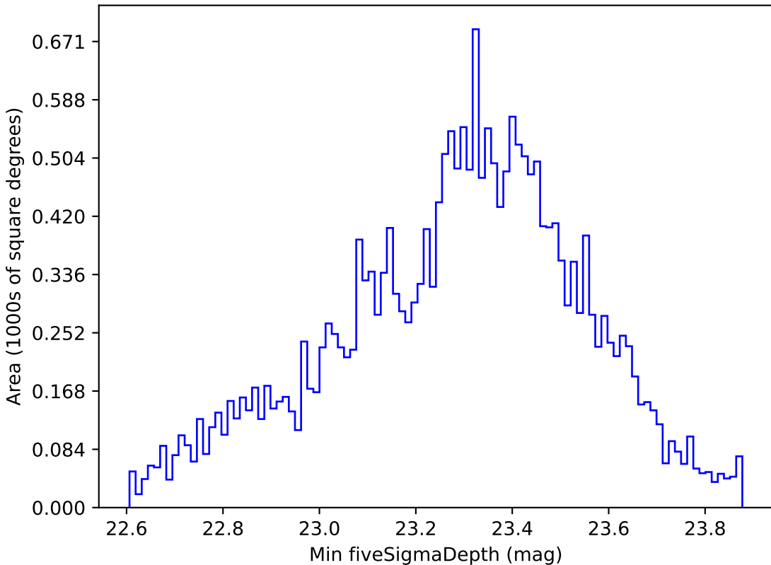
baseline_v2.1_10yrs Yr 1 u band: Min fiveSigmaDepth
