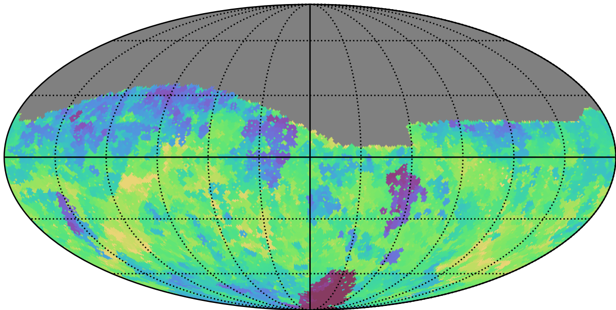
baseline_v2.1_10yrs Yr 1 r band: Min fiveSigmaDepth
