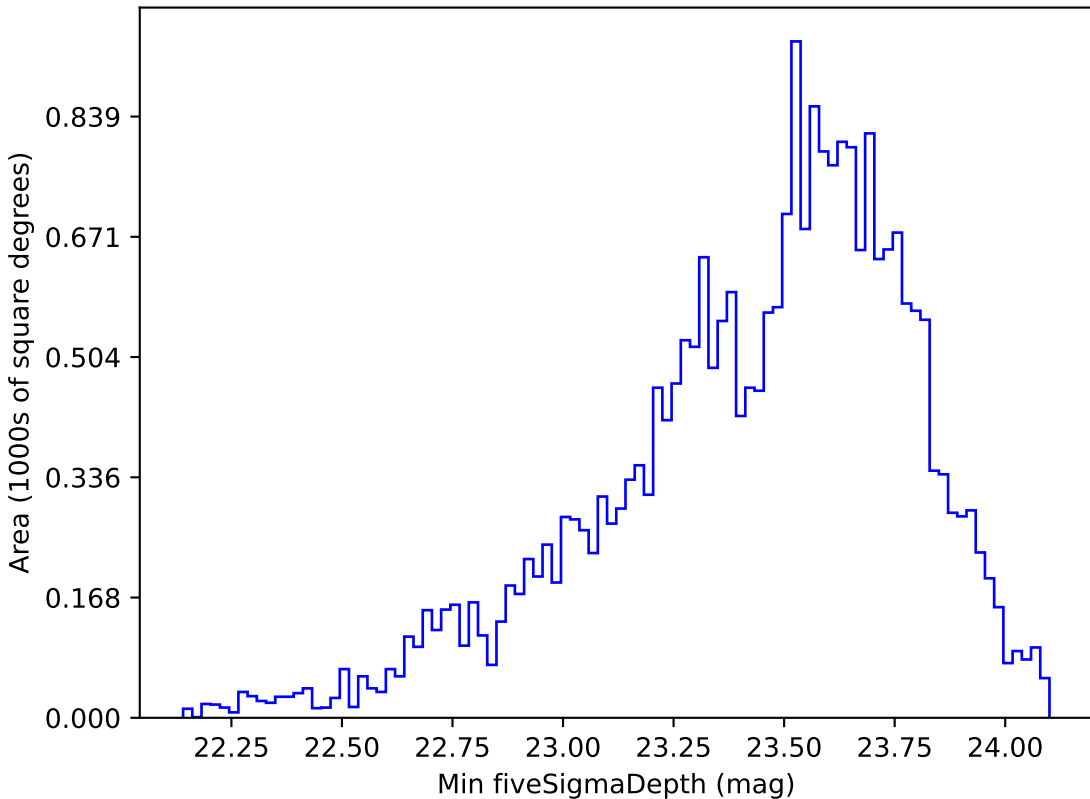
baseline_v2.1_10yrs Yr 1 r band: Min fiveSigmaDepth
