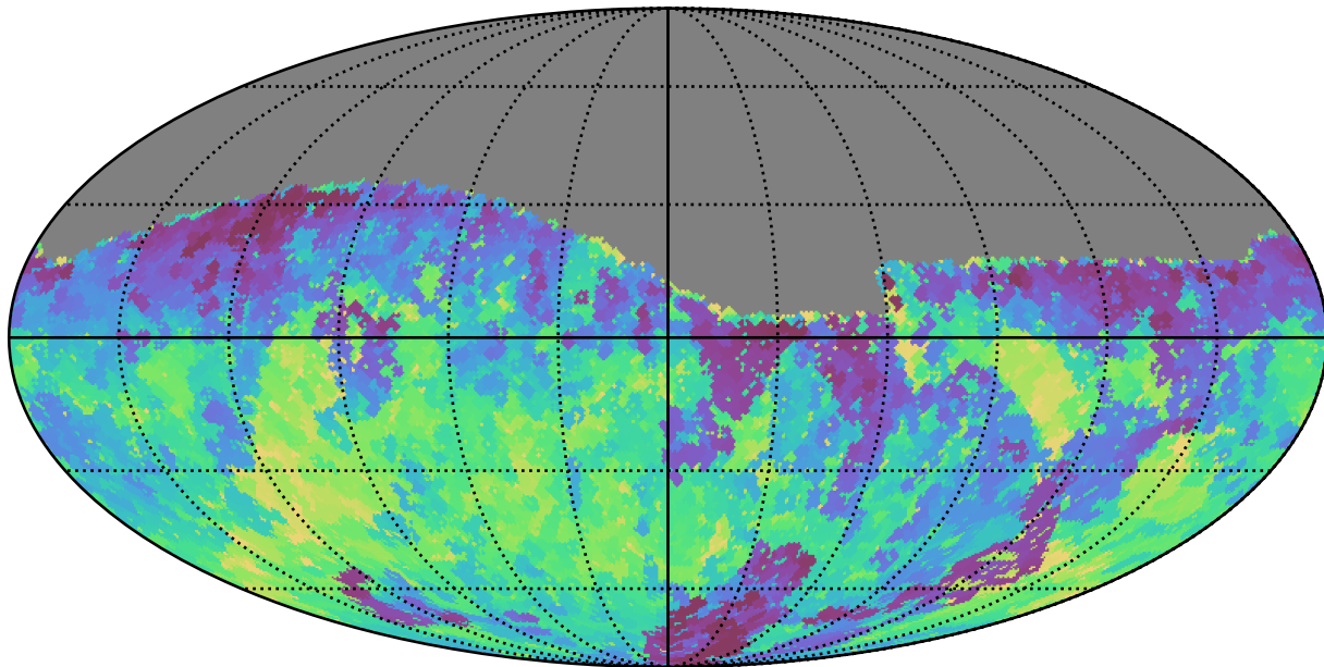
baseline_v2.1_10yrs Yr 1 i band: Min fiveSigmaDepth
