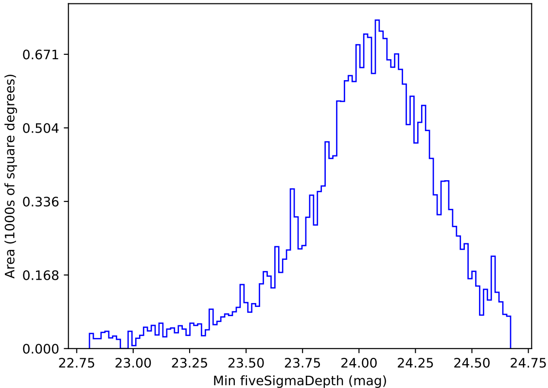
baseline_v2.1_10yrs Yr 1 g band: Min fiveSigmaDepth
