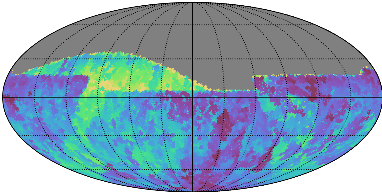
baseline_v2.1_10yrs Yr 1 all bands: Min fiveSigmaDepth
