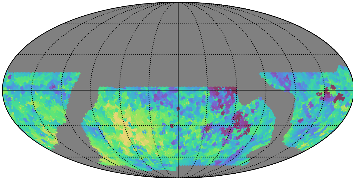
baseline_v2.1_10yrs WFD z band: Min fiveSigmaDepth
