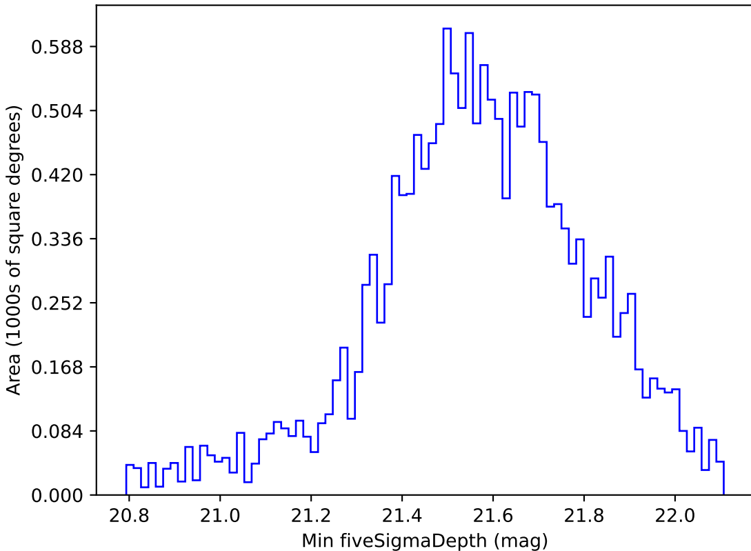
baseline_v2.1_10yrs WFD z band: Min fiveSigmaDepth
