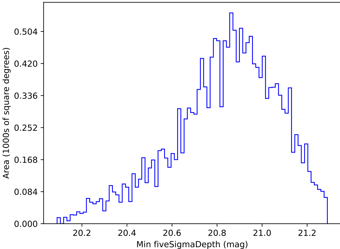
baseline_v2.1_10yrs WFD y band: Min fiveSigmaDepth
