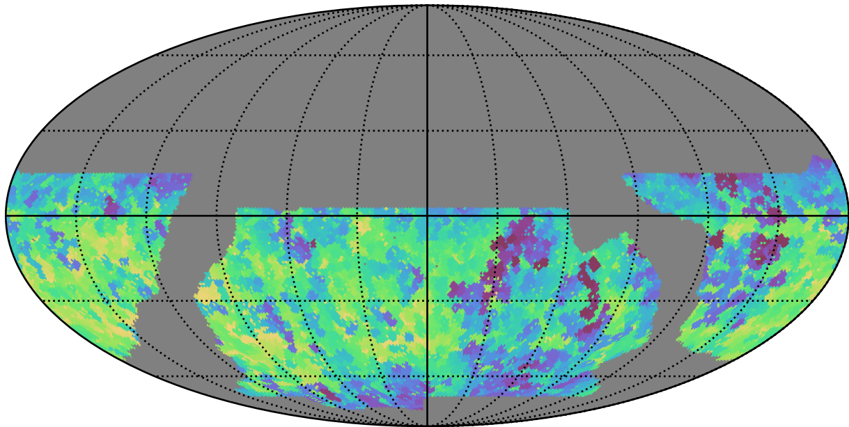
baseline_v2.1_10yrs WFD u band: Min fiveSigmaDepth
