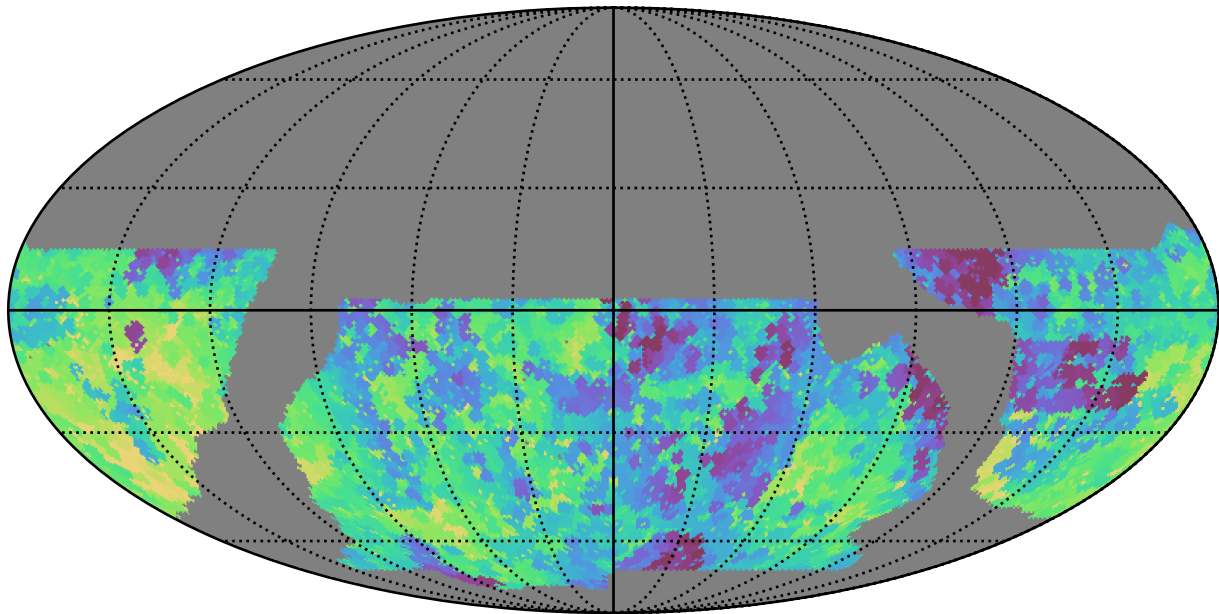
baseline_v2.1_10yrs WFD r band: Min fiveSigmaDepth
