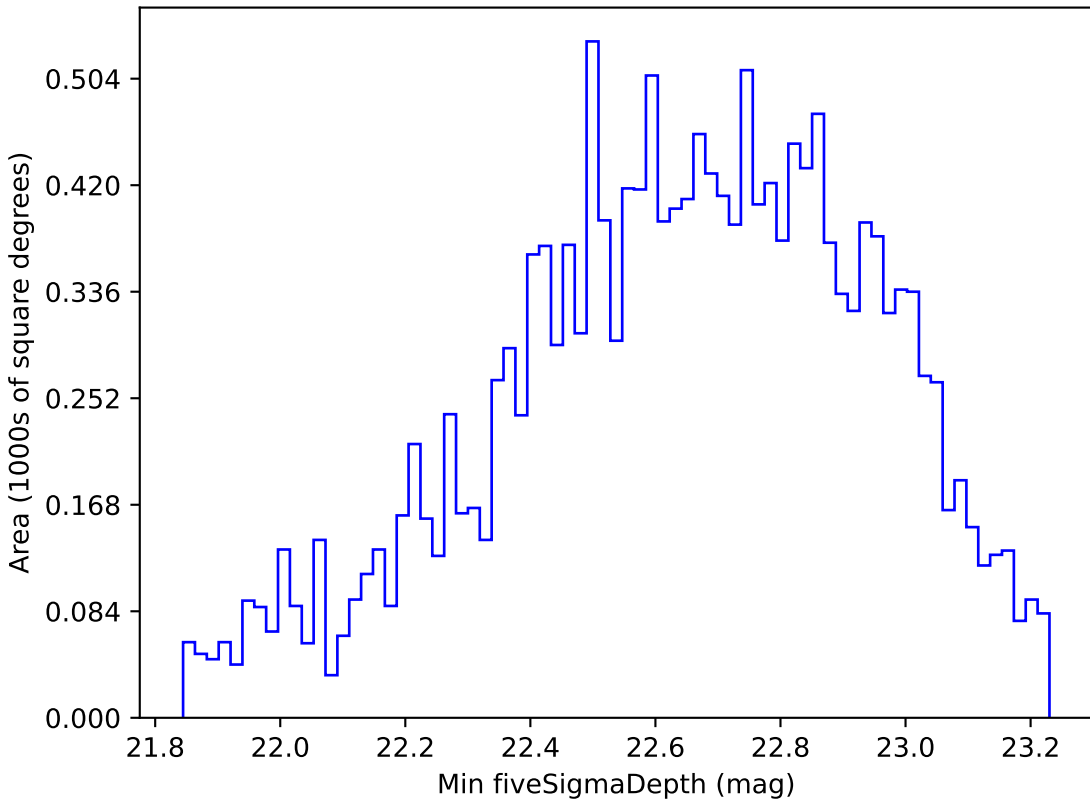
baseline_v2.1_10yrs WFD r band: Min fiveSigmaDepth
