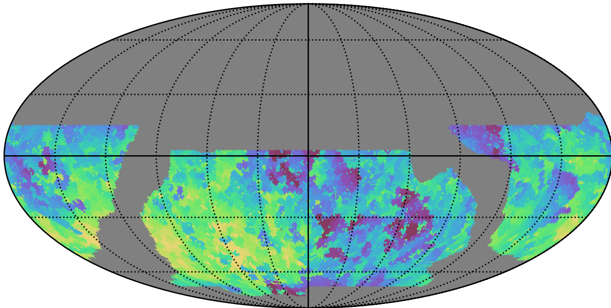
baseline_v2.1_10yrs WFD i band: Min fiveSigmaDepth
