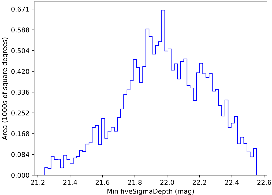
baseline_v2.1_10yrs WFD i band: Min fiveSigmaDepth
