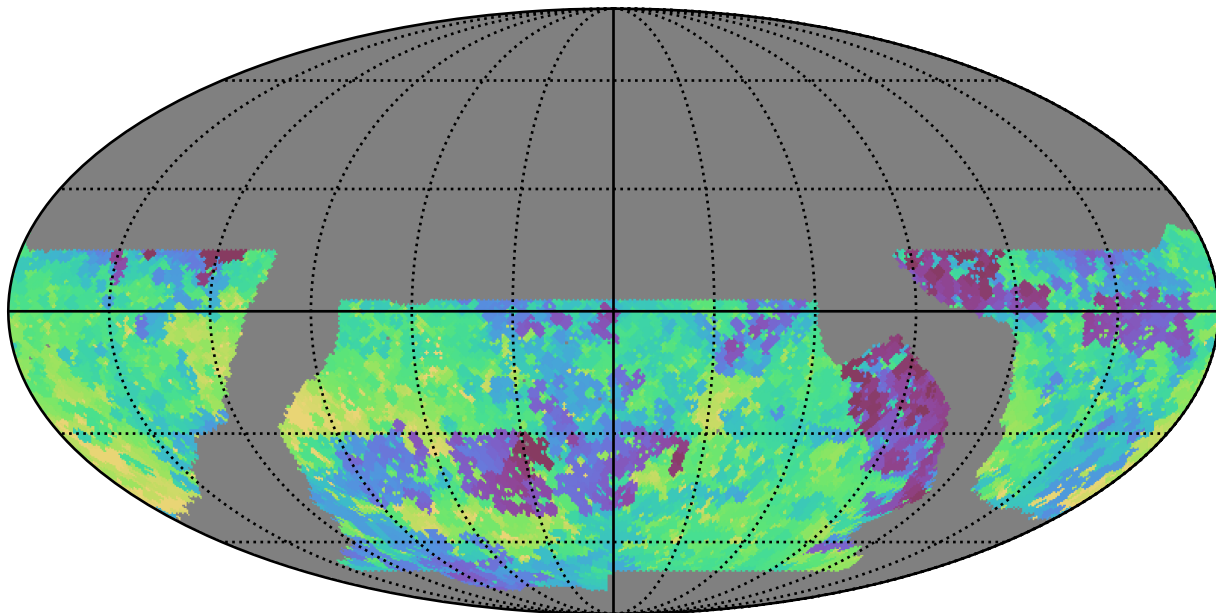
baseline_v2.1_10yrs WFD g band: Min fiveSigmaDepth
