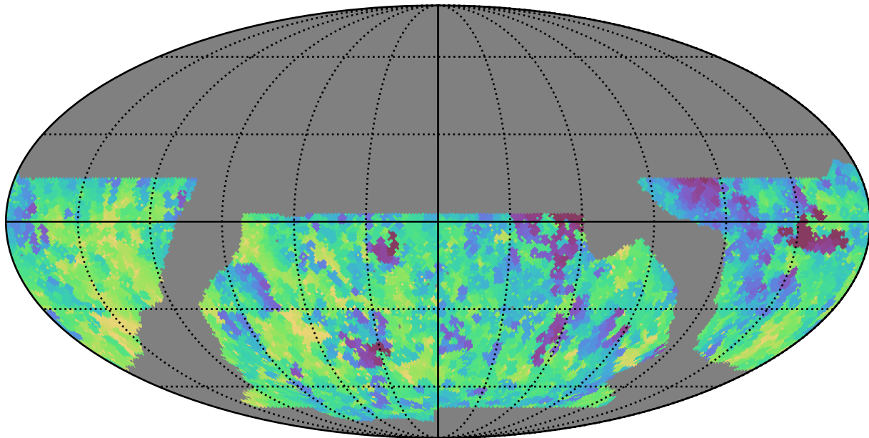
baseline_v2.1_10yrs WFD all bands: Min fiveSigmaDepth
