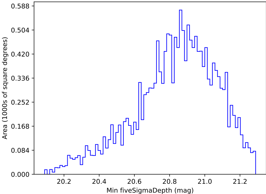
baseline_v2.1_10yrs WFD all bands: Min fiveSigmaDepth
