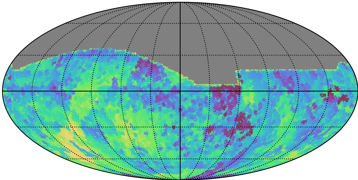
baseline_v2.1_10yrs All sky z band: Min fiveSigmaDepth
