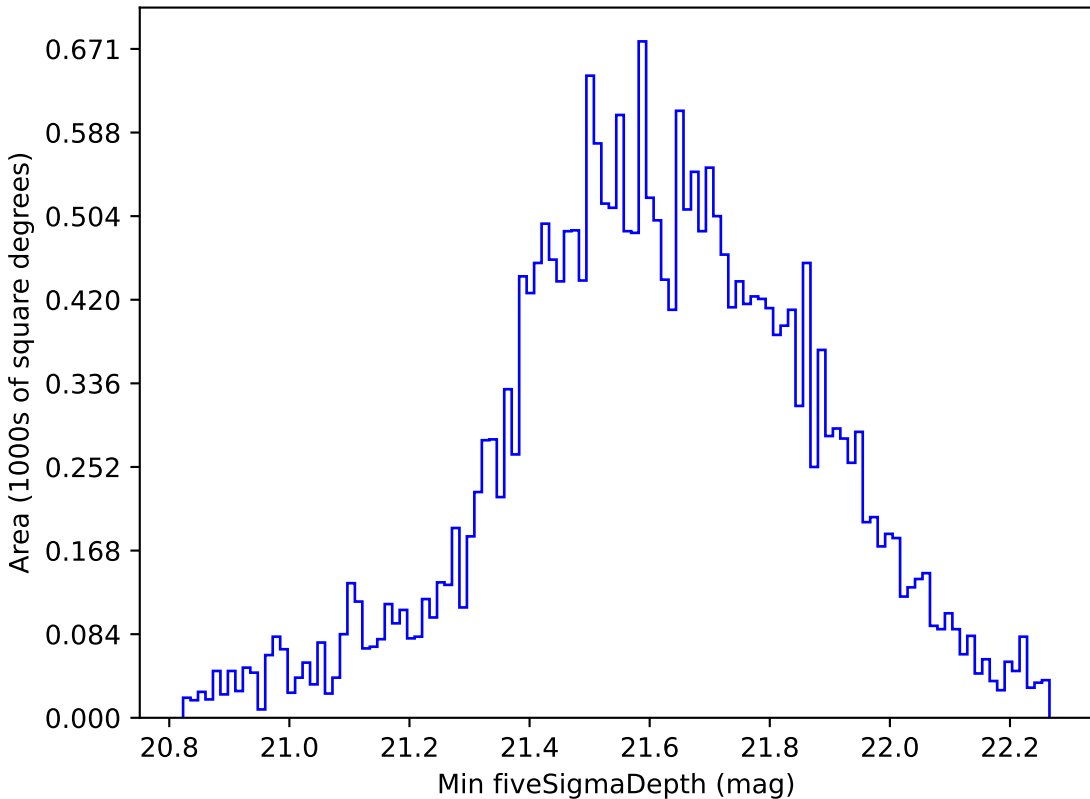
baseline_v2.1_10yrs All sky z band: Min fiveSigmaDepth
