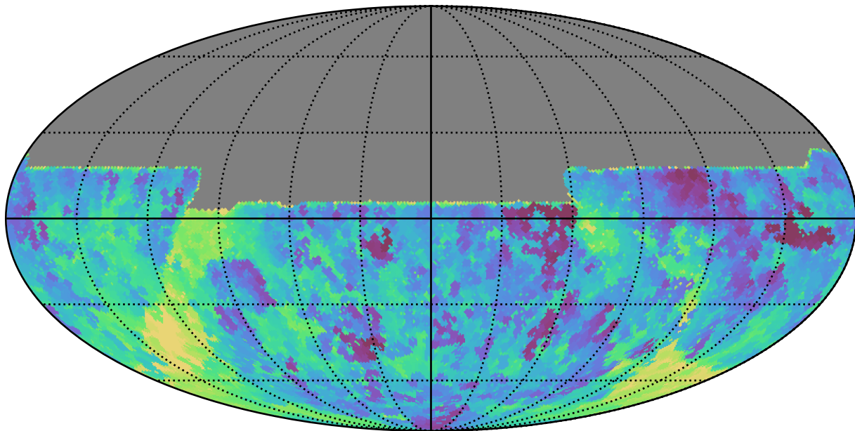
baseline_v2.1_10yrs All sky y band: Min fiveSigmaDepth
