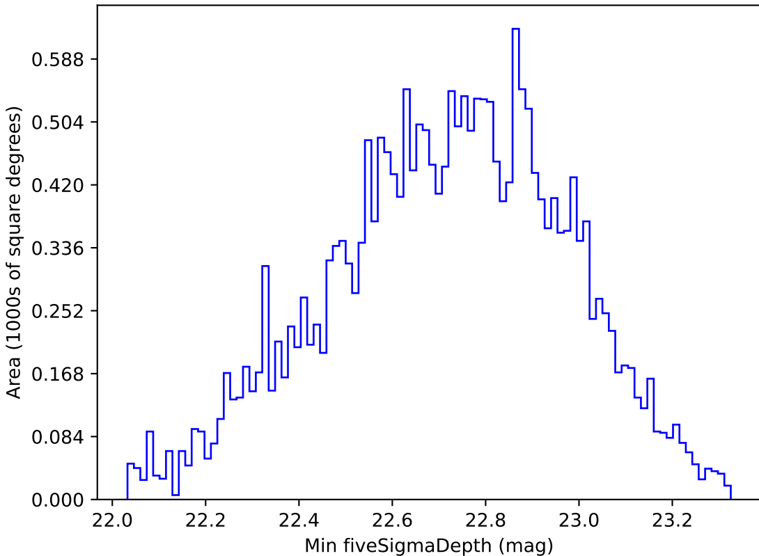
baseline_v2.1_10yrs All sky u band: Min fiveSigmaDepth
