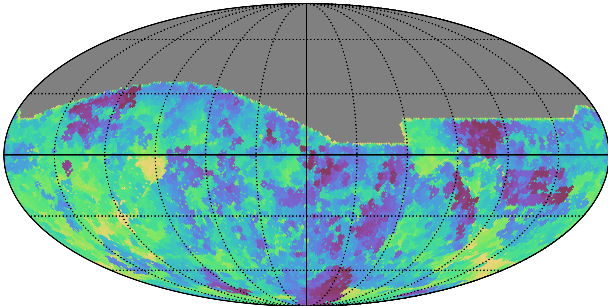
baseline_v2.1_10yrs All sky r band: Min fiveSigmaDepth
