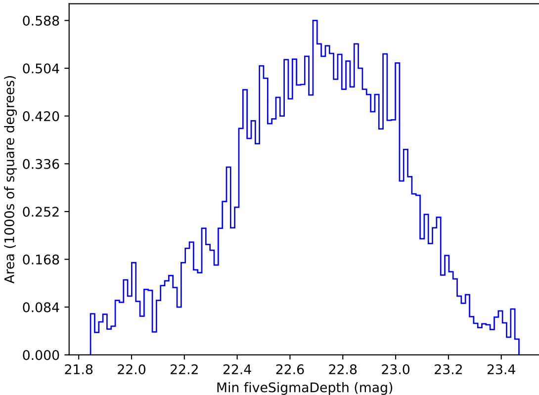
baseline_v2.1_10yrs All sky r band: Min fiveSigmaDepth
