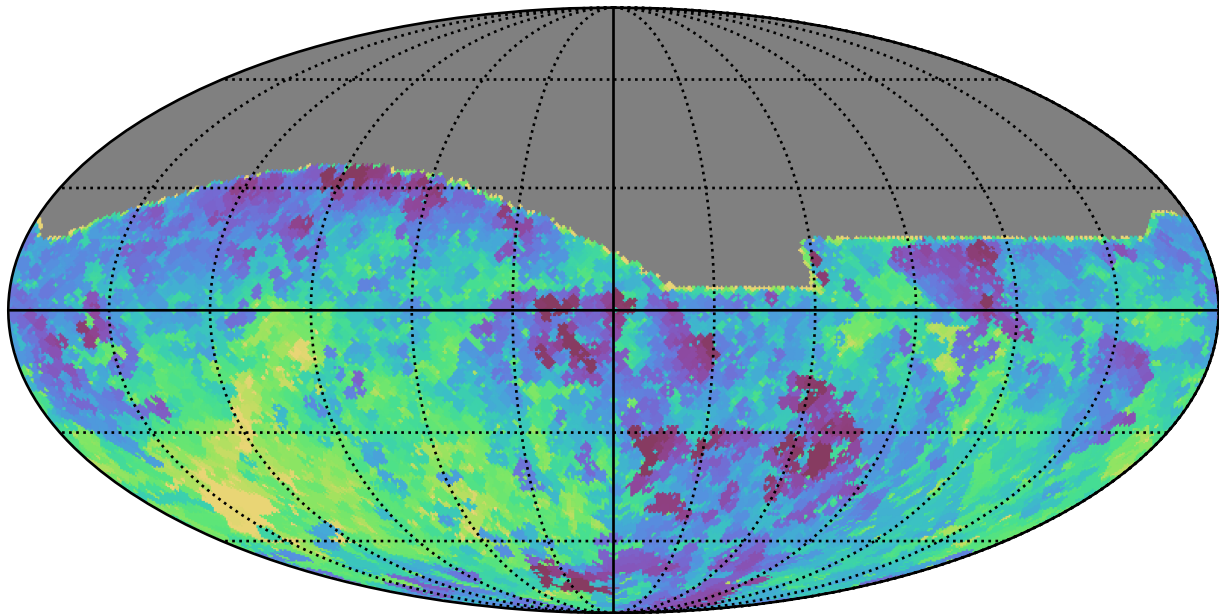
baseline_v2.1_10yrs All sky i band: Min fiveSigmaDepth
