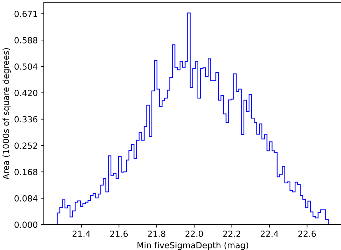
baseline_v2.1_10yrs All sky i band: Min fiveSigmaDepth
