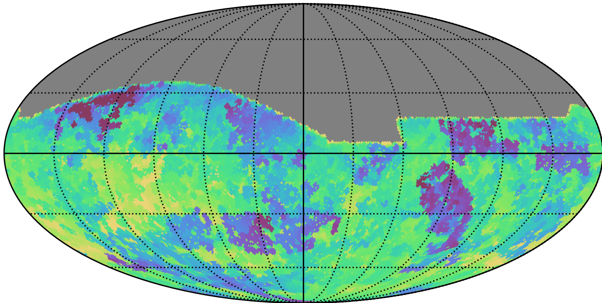
baseline_v2.1_10yrs All sky g band: Min fiveSigmaDepth
