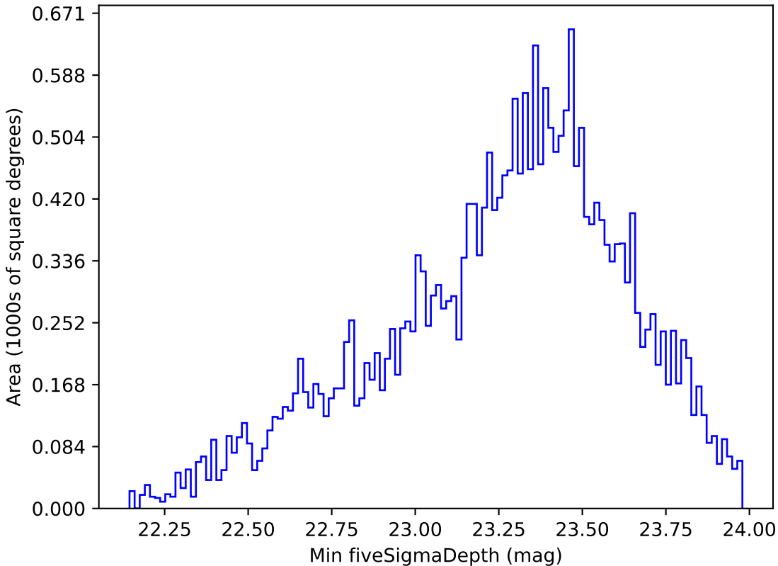
baseline_v2.1_10yrs All sky g band: Min fiveSigmaDepth
