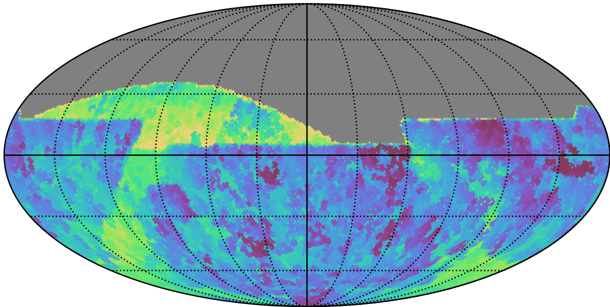
baseline_v2.1_10yrs All sky all bands: Min fiveSigmaDepth
