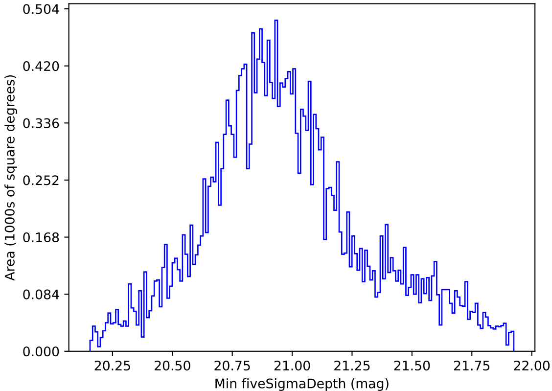
baseline_v2.1_10yrs All sky all bands: Min fiveSigmaDepth
