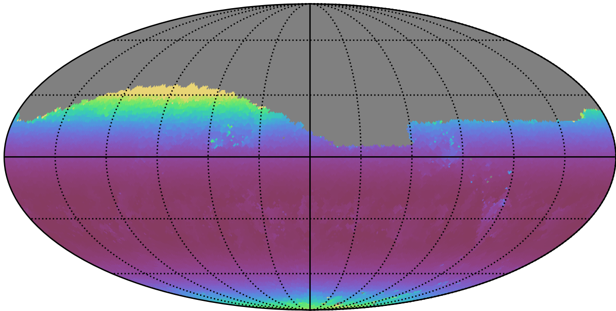
baseline_v2.1_10yrs Yr 1 z band: Min airmass
