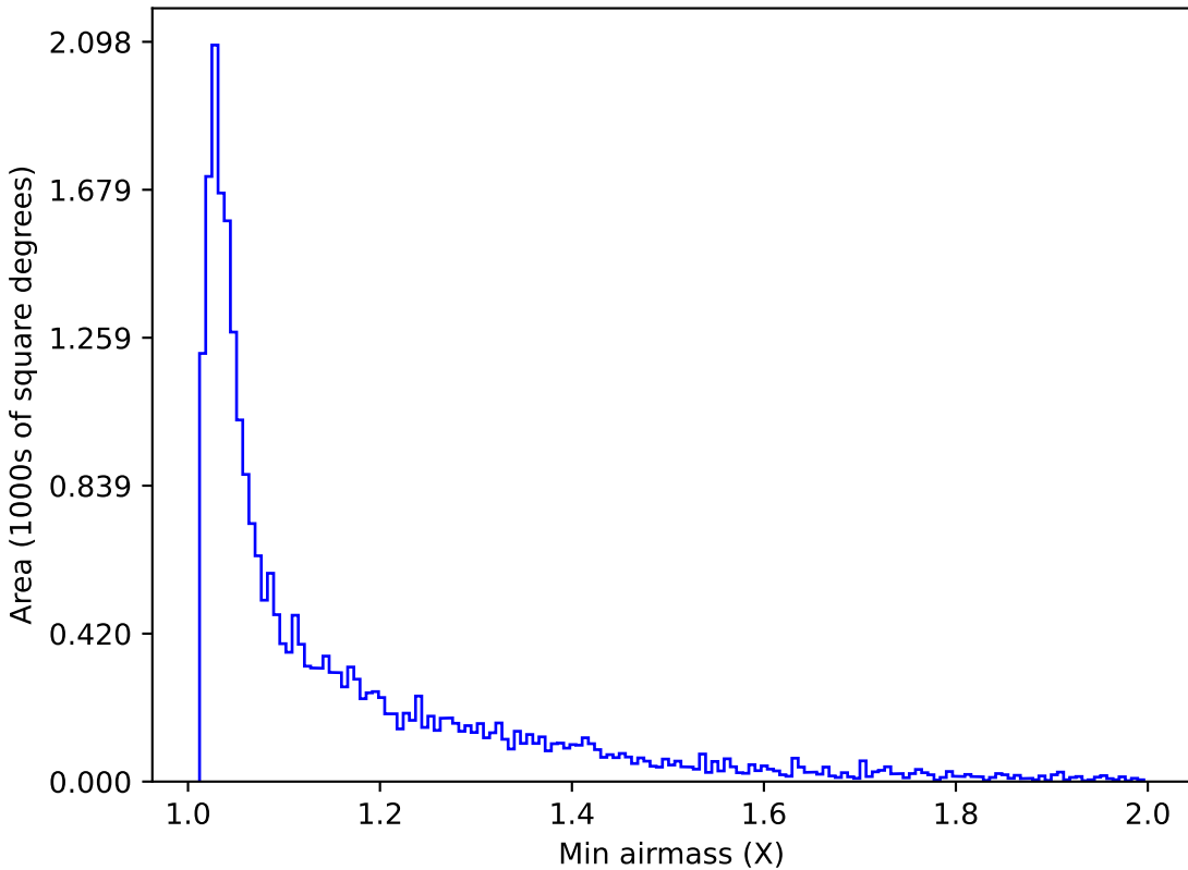
baseline_v2.1_10yrs Yr 1 z band: Min airmass
