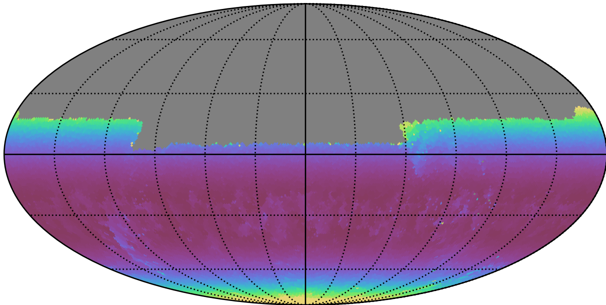
baseline_v2.1_10yrs Yr 1 y band: Min airmass
