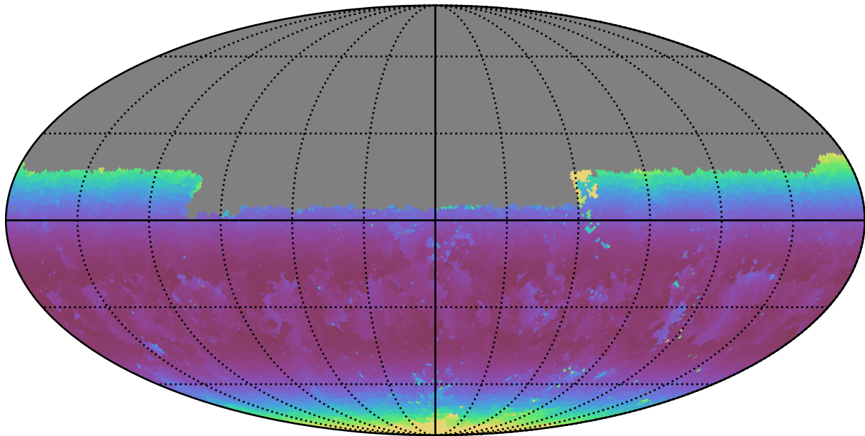
baseline_v2.1_10yrs Yr 1 u band: Min airmass
