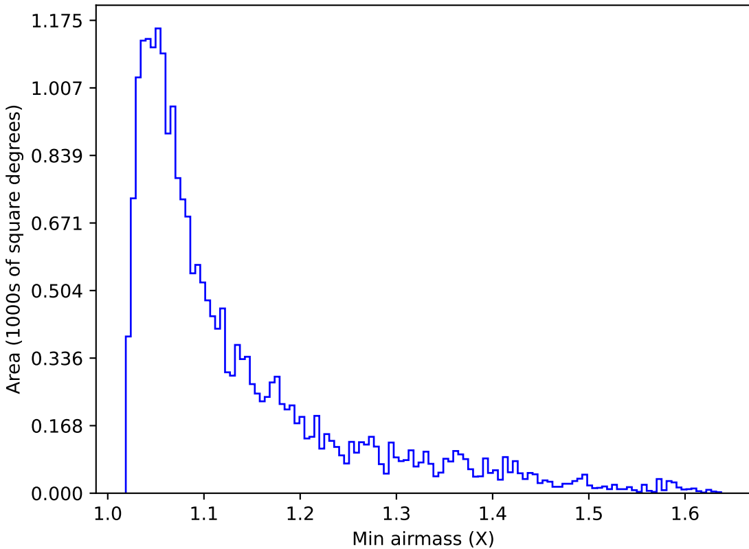
baseline_v2.1_10yrs Yr 1 u band: Min airmass
