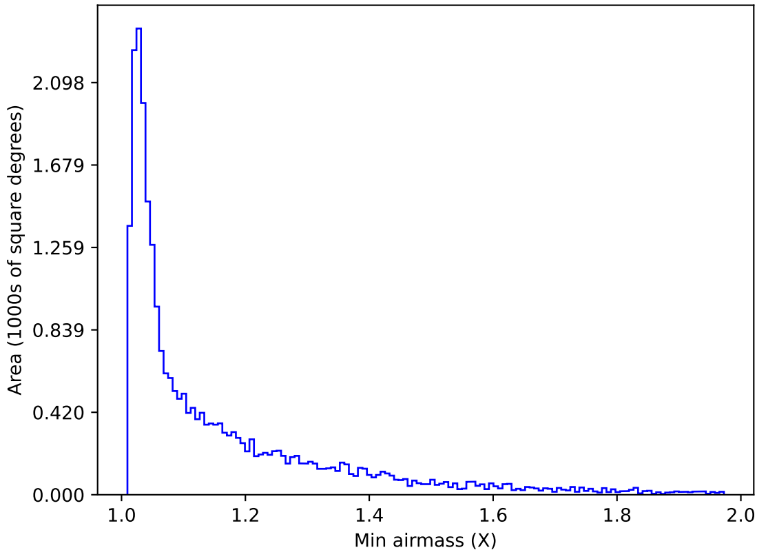
baseline_v2.1_10yrs Yr 1 r band: Min airmass
