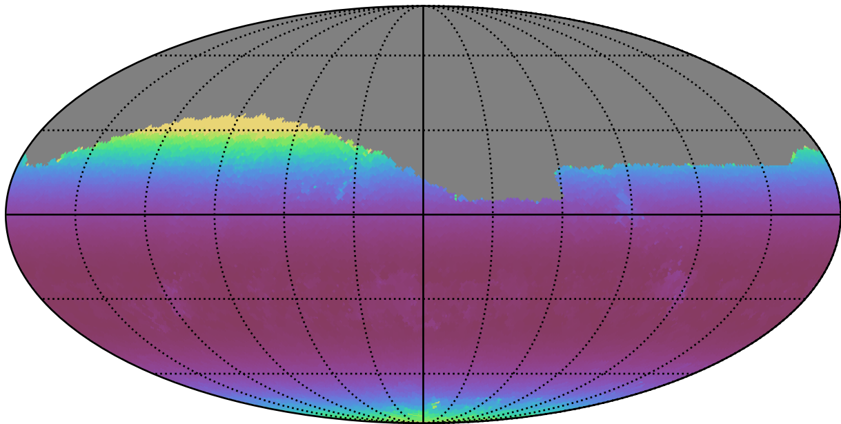
baseline_v2.1_10yrs Yr 1 i band: Min airmass
