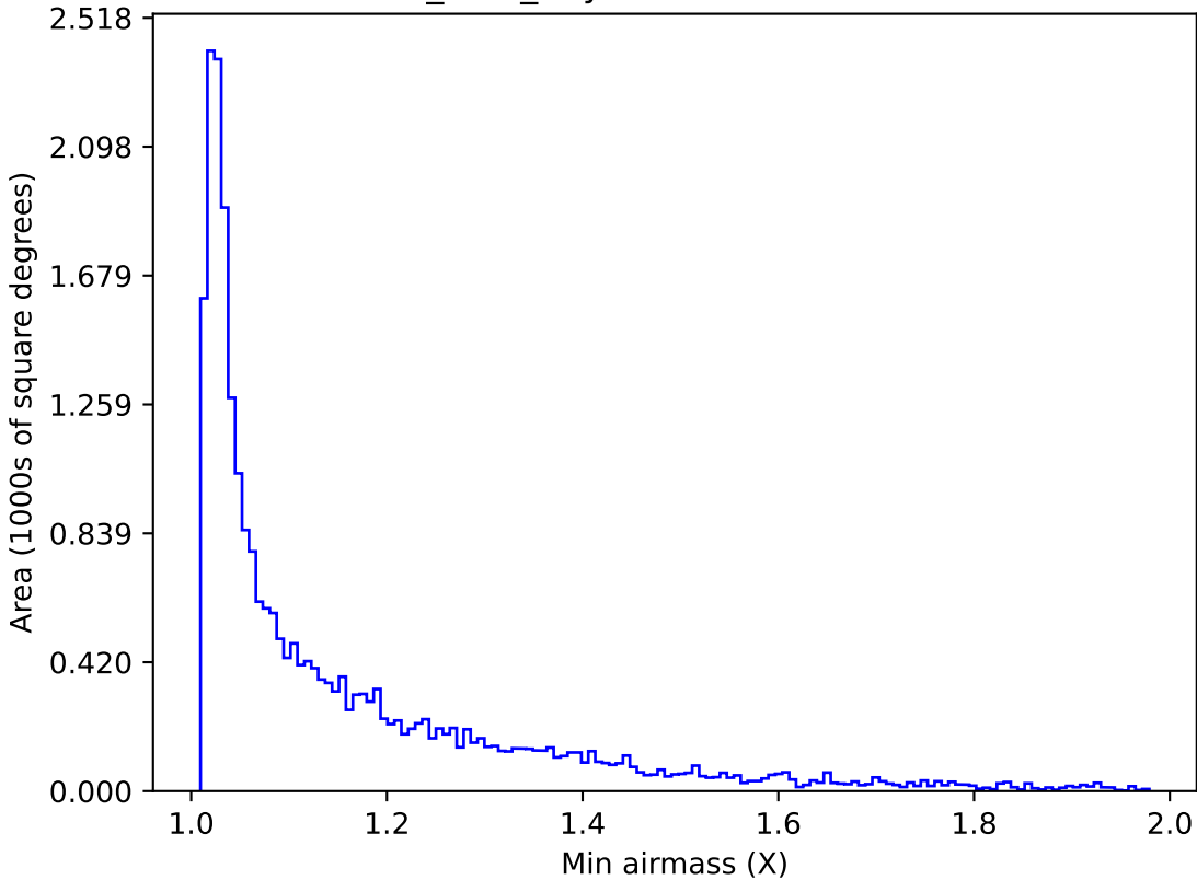
baseline_v2.1_10yrs Yr 1 i band: Min airmass
